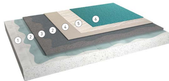
1 concrete substrate, 2 primer, 3 floor screed, 4 self-levelling compound, 5 carpet adhesive, 6 carpet
