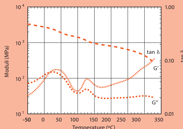
Fig. 3.2.3 • Dynamic Mechanical Analysis Vectra® S135
