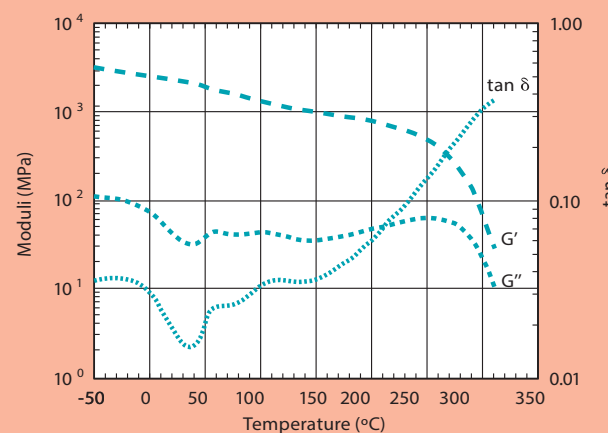
Fig. 3.2.2 • Dynamic Mechanical Analysis Vectra® E130i
