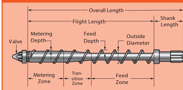
Fig. 6.1.1 • Metering Type Screws Recommended for Processing Vectra® LCP
