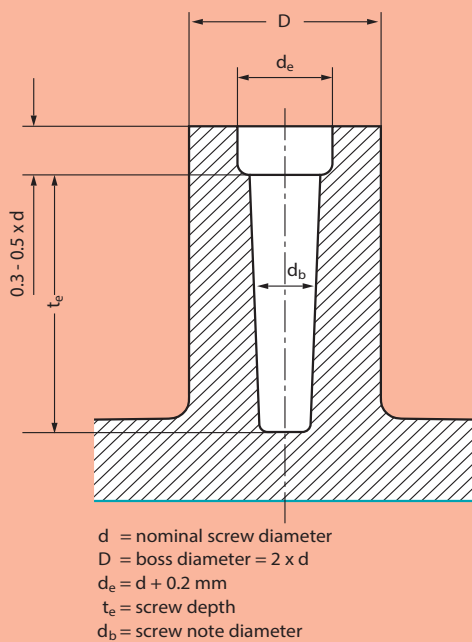
Fig. 9.2.7 Boss for EJOT PT® K Screw
