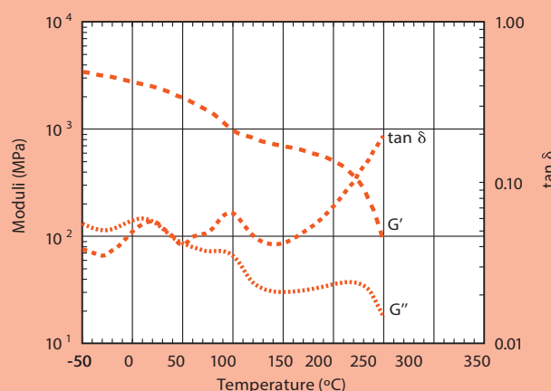
Fig. 3.2.1 • Dynamic Mechanical Analysis Vectra® A130
