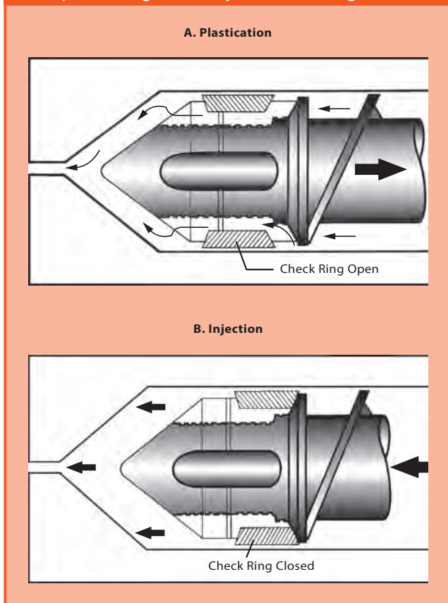
Fig. 6.1.2 • Check Ring Non-Return Valve Used on Reciprocoating Screw Injection Molding Machine
