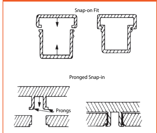
Fig. 5.4 • Snap-on/Snap-in Fits
