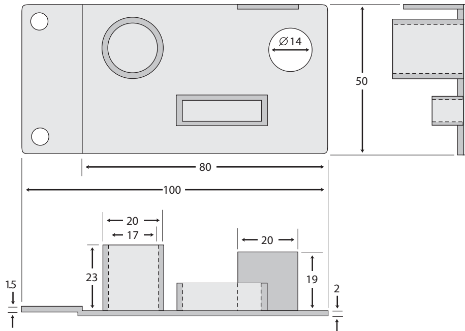
Figure 7 Specifications for warpage sample, dimensions in millimeters
