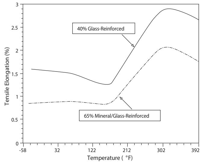
Figure 6 Temperature dependence of tensile elongation at break
