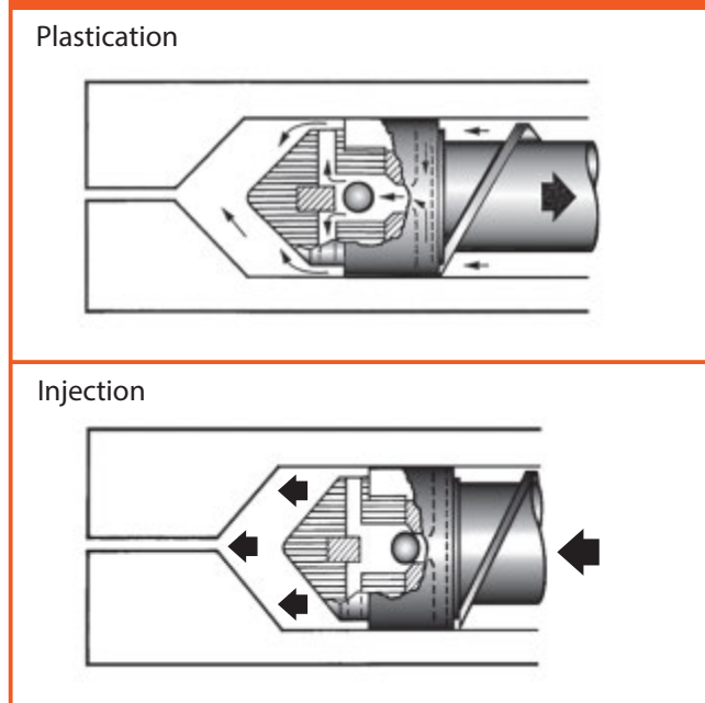
Fig. 3.5 • Internal Ball Check Nonreturn Valve Used on Reciprocating Screw Injection Molding Machines
