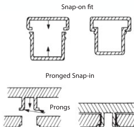
Fig. 5.4 • Snap-on/Snap-in Fits
