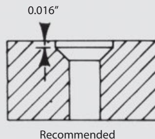
Fig. 4.1 • Chamfered Hole for Machine Tapping
