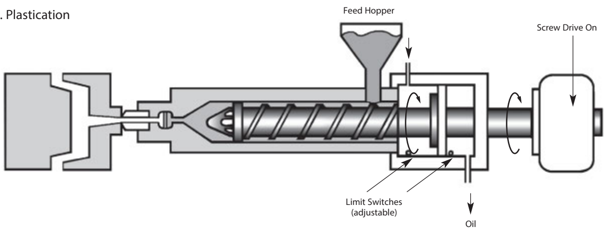
Fig. 3.1 • Molding Sequence, Single Stage Reciprocating Screw Injection Molding Machine
