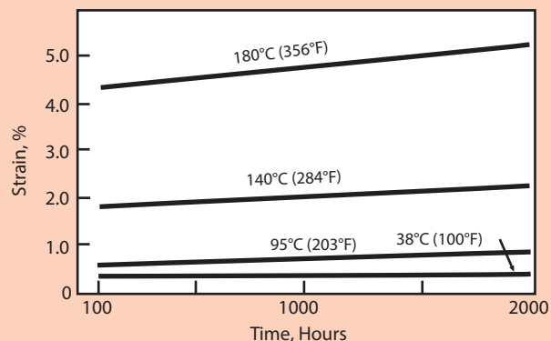
Fig. 2.24 • Flexural Creep at 2000 psi Maximum Stress for Glass Reinforced Celanex® 3200
