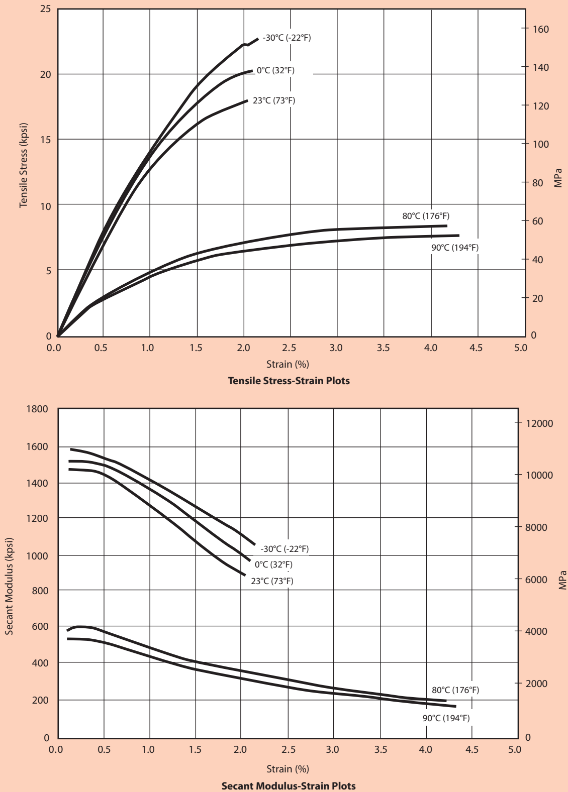
Fig. 2.14 • Typical Tensile Stress and Secant Modulus Plots at Different Temperatures for Glass/Mineral Reinforced Celanex® 6500
